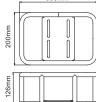
ALUMINUM FRONT CARRIER Dimension 300mm
